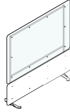
Clear top panel, no cutouts; opaque bottom panel 72"W x 72"H
