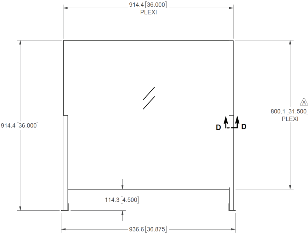
View 1. Elevation
