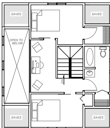
2nd Floor Plan Not to Scale
