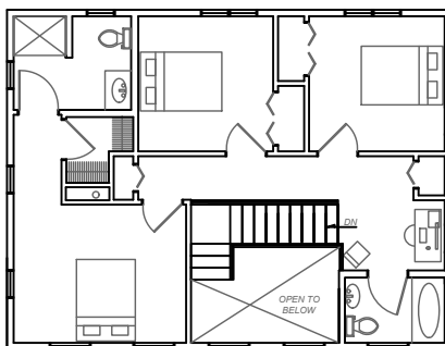
2nd Floor Plan Not to Scale
