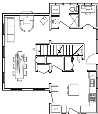
1st Floor Plan Not to Scale
