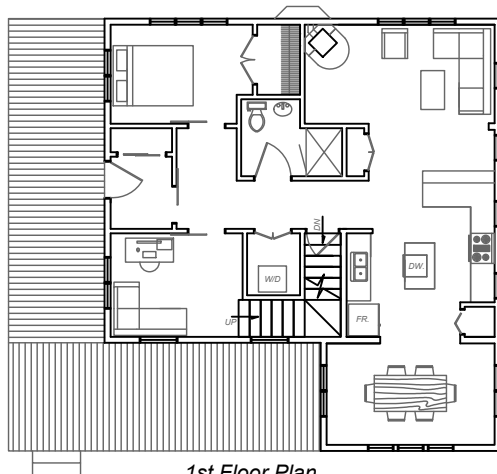
1st Floor Plan Not to Scale
