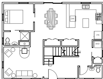
1st Floor Plan Not to Scale
