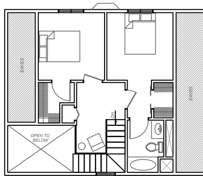
2nd Floor Plan Not to Scale
