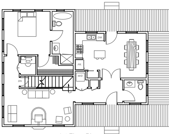
1st Floor Plan Not to Scale
