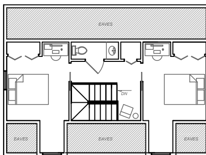
2nd Floor Plan Not to Scale
